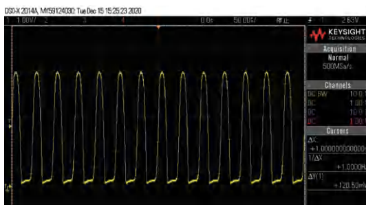
▲ Common Load Performance-Self-excitation
